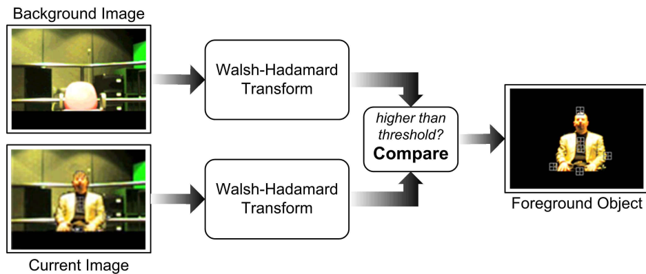
Fig. 3. Extracting the user’s image from his background
